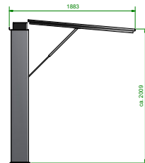
Lefthand View 1:20
