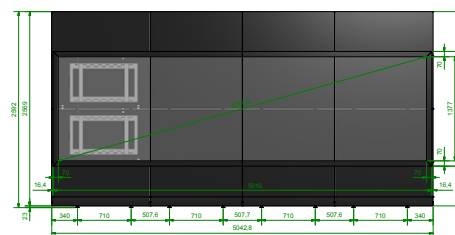
Front View 1:20
