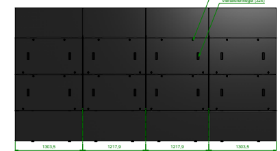
Back View 1:20
