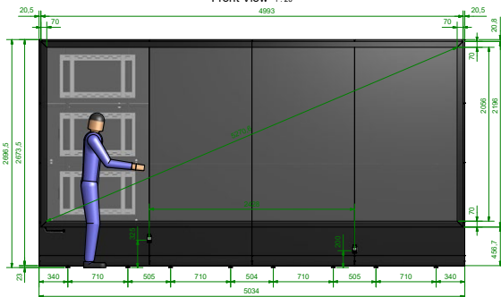
Front View 1:20
