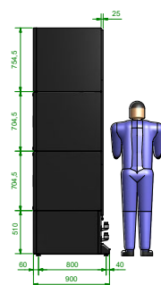
Lefthand View 1:20
