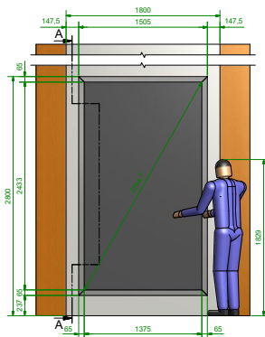
Front View 1:20
